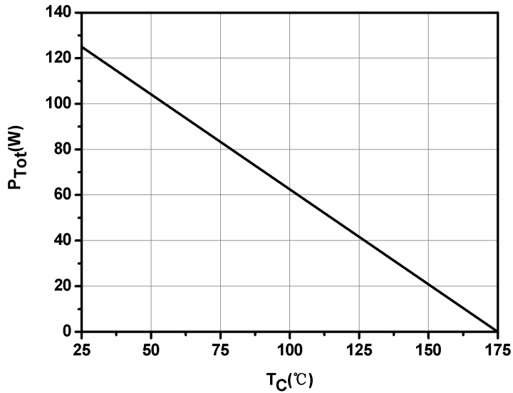
Fig.5-Power Derating
